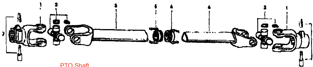
PTO Shaft
